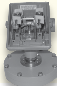
Dual Switch, Low Water Column Differential Pressure Model
